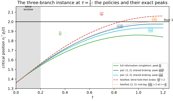
Figure 1: The audited policies on the critical coordinate n_j^T p_j(t) at \tau = \frac{1}{5} , every peak the exact rational of the text: the full-information singleton peaks at \frac{93}{50} ; the pair policies peak below the floor ( \frac{12345}{6250} , \frac{2419}{1250} , slacks \frac{31}{1250} and \frac{81}{1250} ); the two falsified variants cross it ( \frac{103}{50} , \frac{2501}{1250} at t = \frac{29}{25} ). Generated by the assertion script paper2.comp.certification.figures.v1.py .
